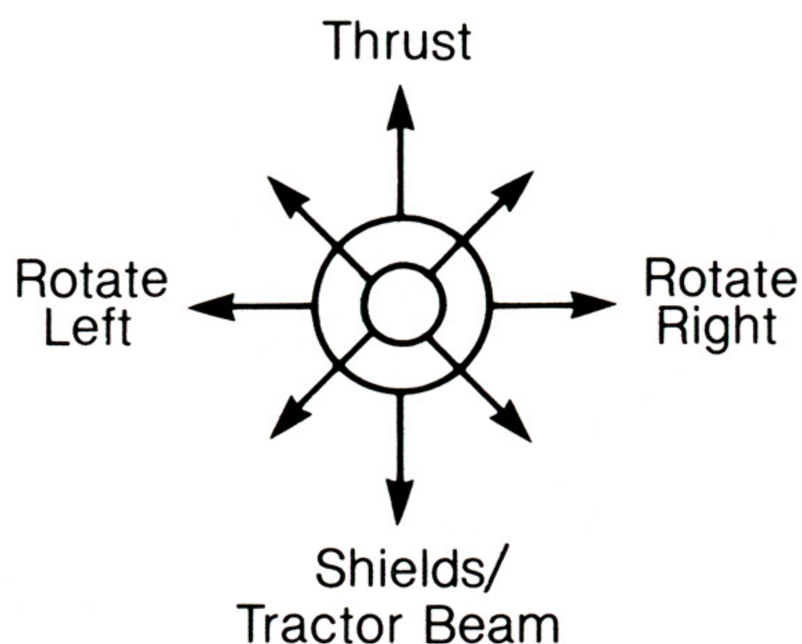
Figure 4—Spaceship Maneuvers
