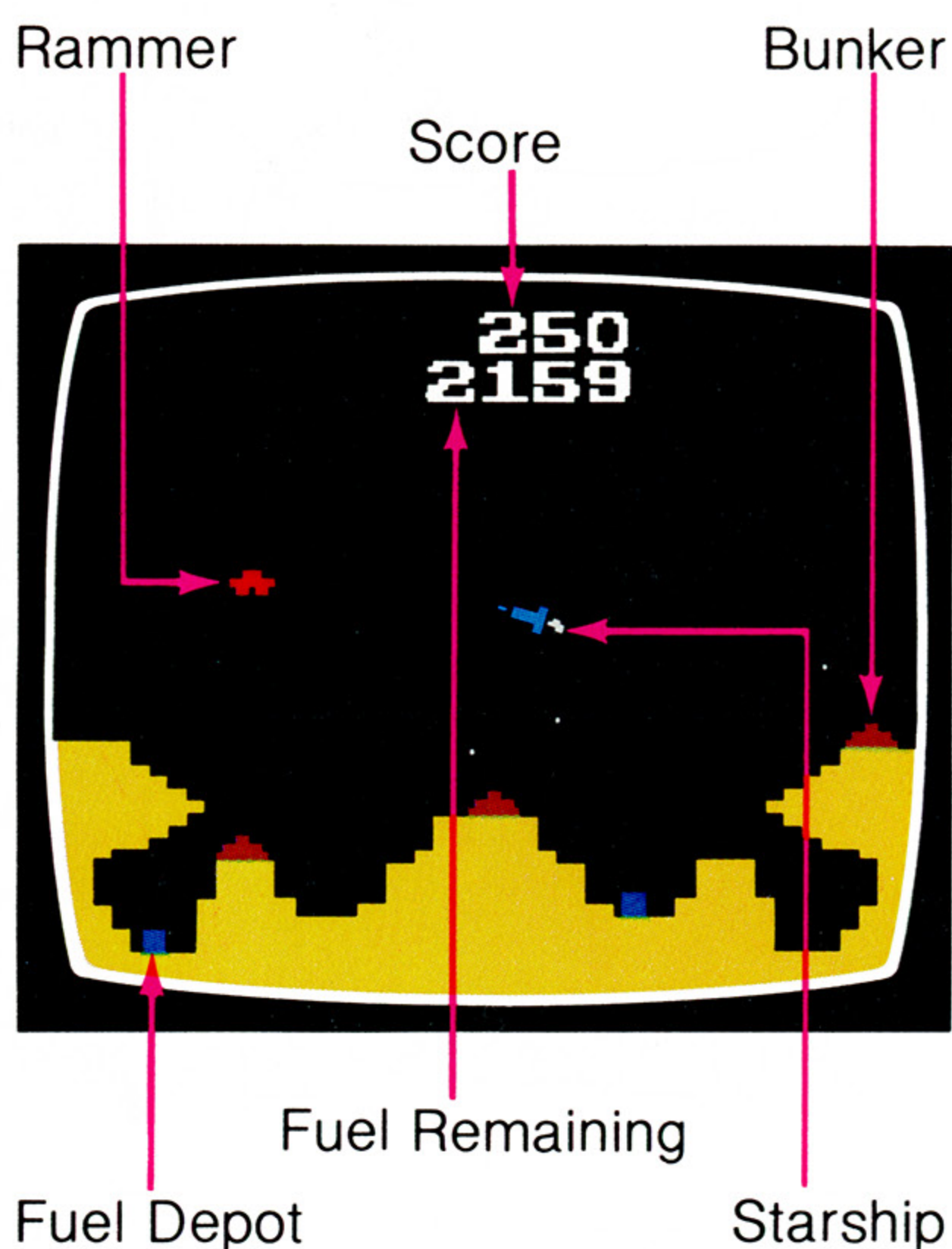
Figure 2—Planet Landscape
