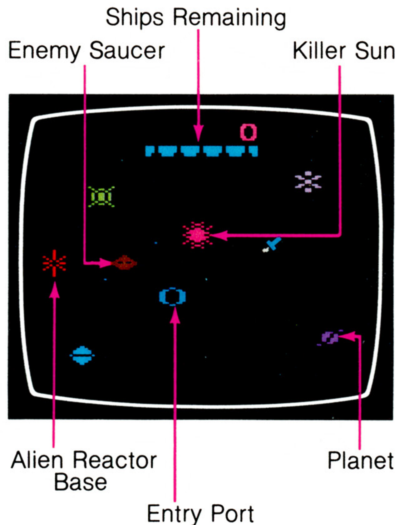
Figure 1 — Solar System
